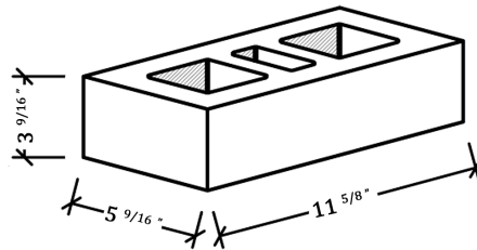
SUMMIT PLANT SIX INCH UNIWALL
