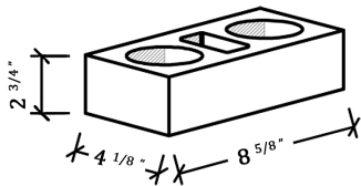
SUMMIT PLANT SUPER QUEEN UNIWALL
